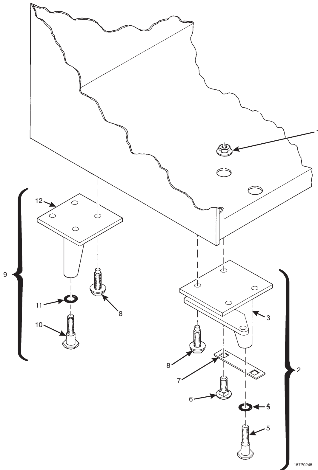
Figure 22. Leg, Leveler, and Leg and Hinge Assemblies
