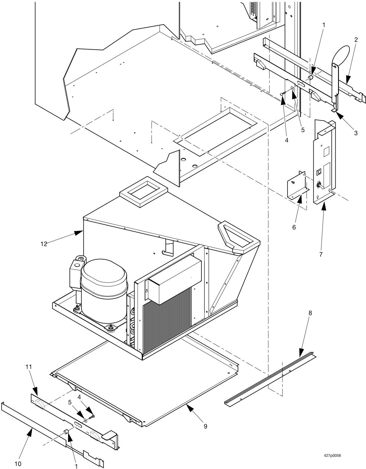
Figure 29. Refrigeration Unit
